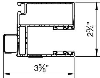
TRACK DETAIL
