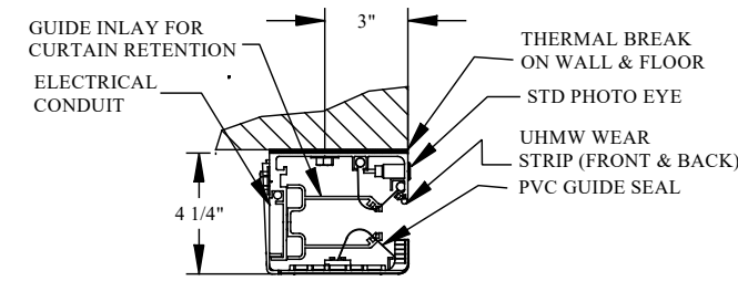
GUIDE SECTION VIEW (DO NOT SCALE)
