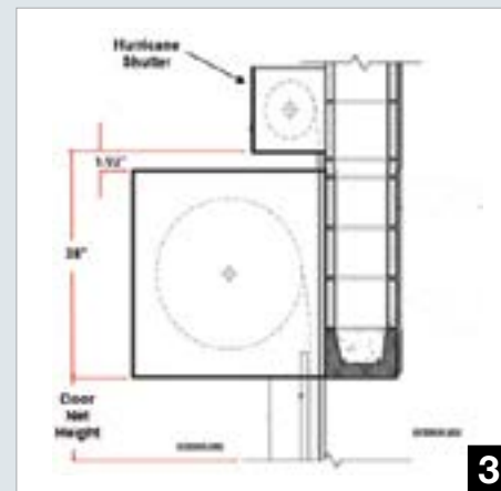
Hurricane Shutter Above Lintel Mount
