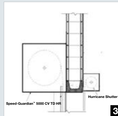
Hurricane Shutter Exterior Mount
